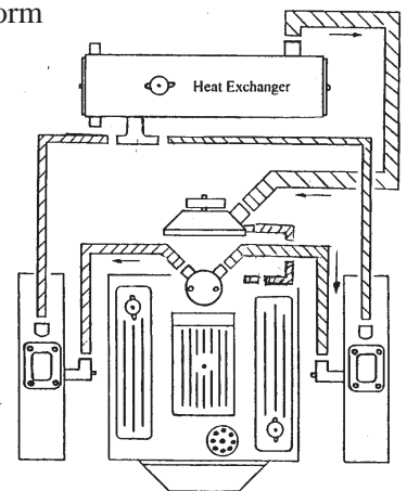
MERCUISER 7.4 ENGINES COOLANT WATER SCHEMATIC FULL SYSTEM
