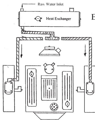
MERCUISER 7.4 ENGINES RAW WATER SCHEMATIC FULL SYSTEM
