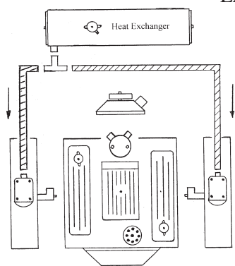
MERCUISER V-6 & V-8 ENGINES RAW WATER SCHEMATIC FULL SYSTEM
