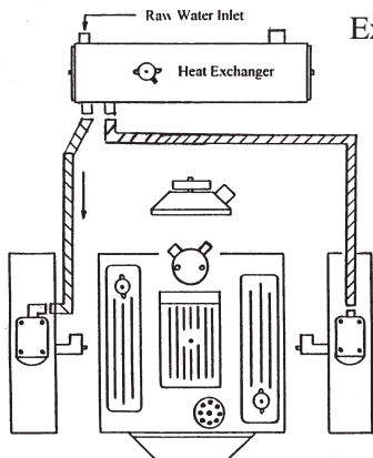
MERCUISER V-6 & V-8 ENGINES RAW WATER SCHEMATIC FULL SYSTEM
