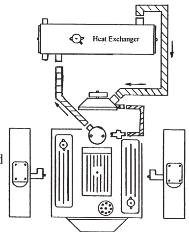
MERCUISER V-6 & V-8 ENGINES. COOLANT WATER SCHEMATIC BLOCK ONLY
