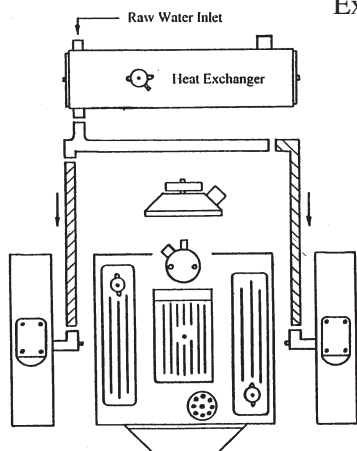
MERCUISER V-6 & V-8 ENGINES RAW WATER SCHEMATIC BLOCK ONLY
